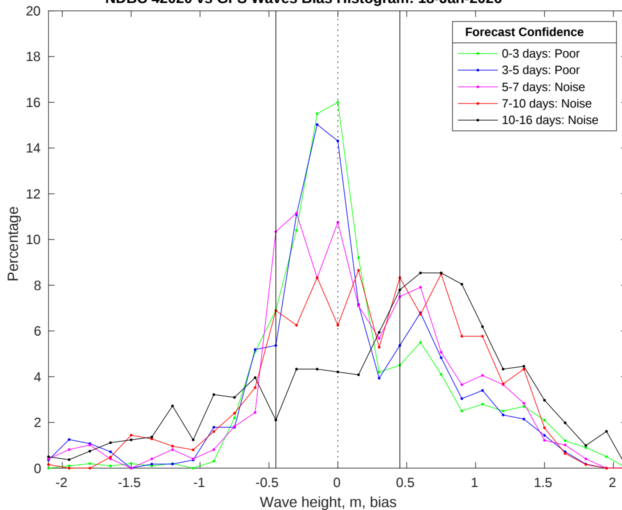
NDBC 42020 vs GFS Waves Bias Histogram: 18-Jan-2026
