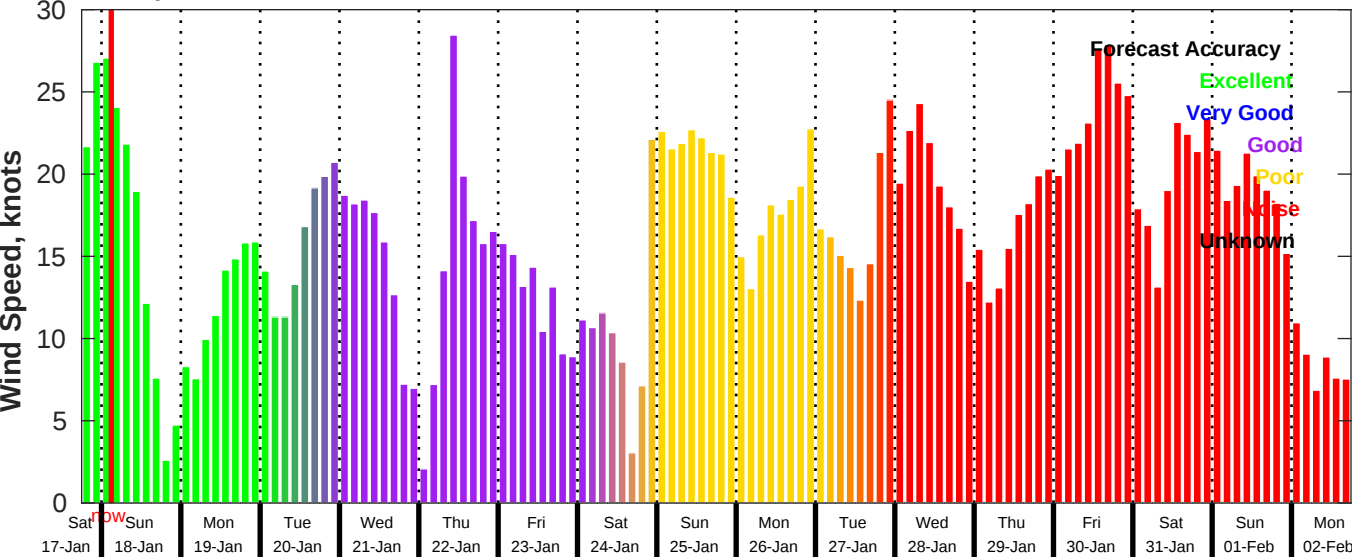
GFS Wind Speed Forecast for NDBC 42020 from 17-Jan-2026 18:00:00 to 02-Feb-2026 18:00:00
