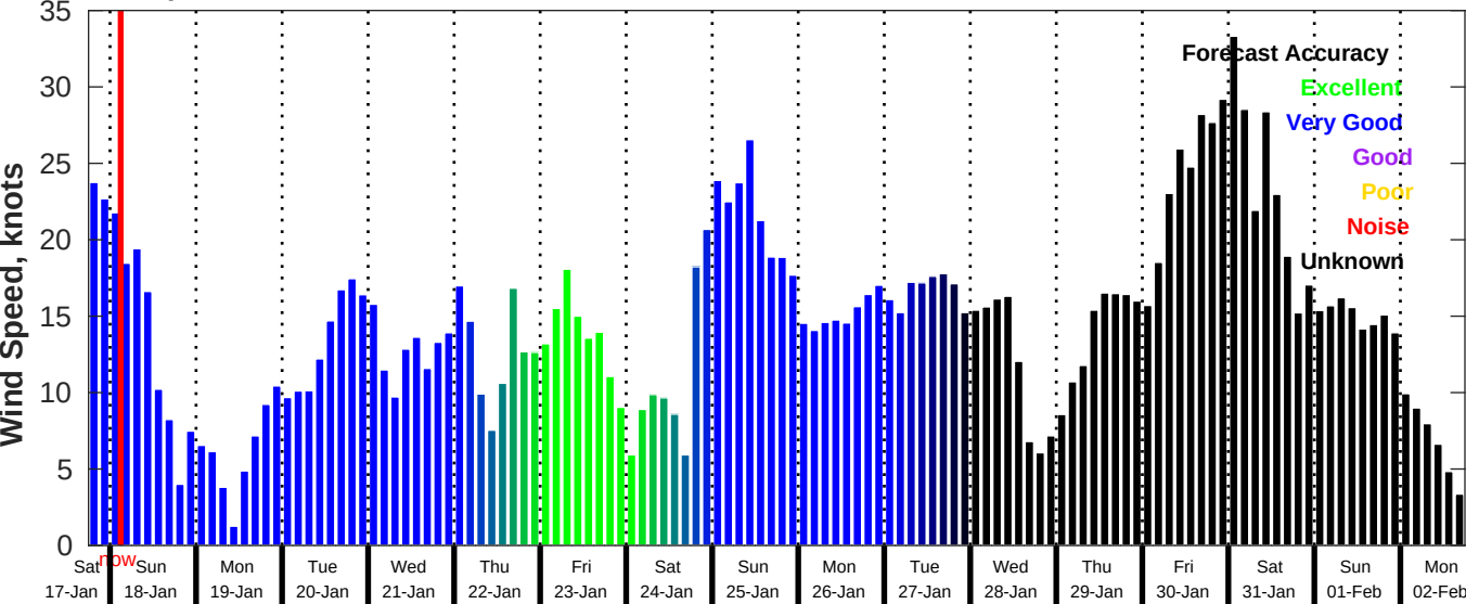
GFS Wind Speed Forecast for NDBC 42035 from 17-Jan-2026 18:00:00 to 02-Feb-2026 18:00:00
