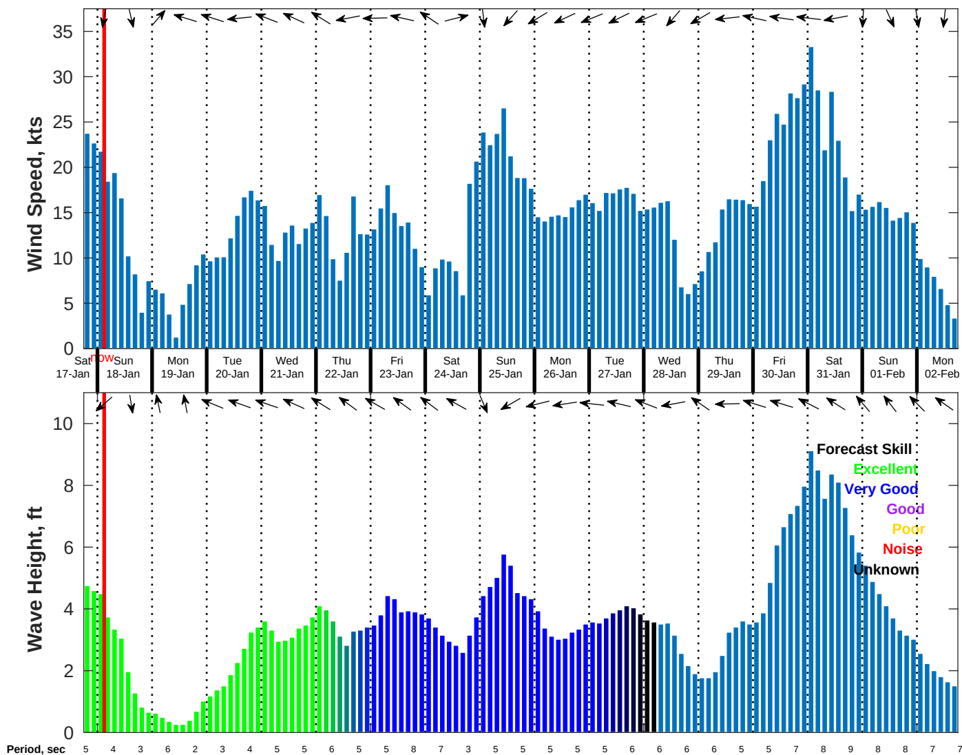
Wind & Wave Forecast for NDBC 42035 from 17-Jan-2026 18:00:00 to 02-Feb-2026 18:00:00
