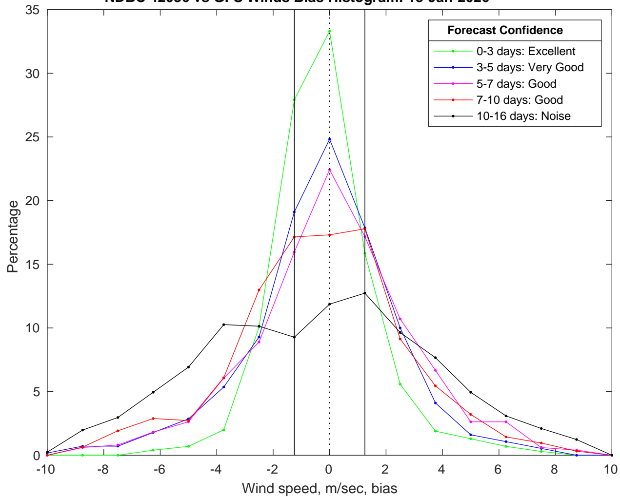
NDBC 42036 vs GFS Winds Bias Histogram: 18-Jan-2026
