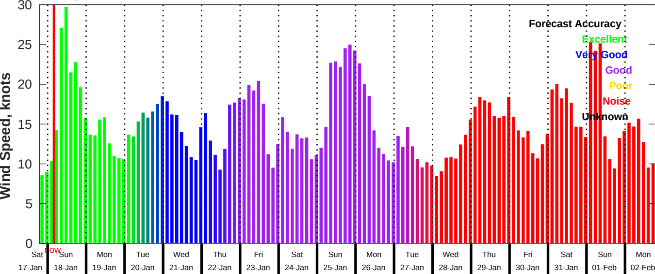
GFS Wind Speed Forecast for NDBC 42036 from 17-Jan-2026 19:00:00 to 02-Feb-2026 19:00:00
