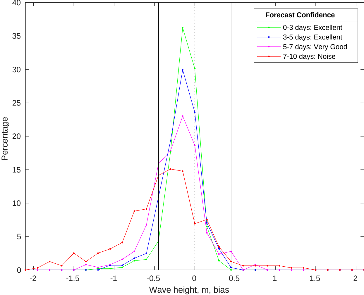
NDBC 42040 vs CMEMS Waves Bias Histogram: 18-Jan-2026
