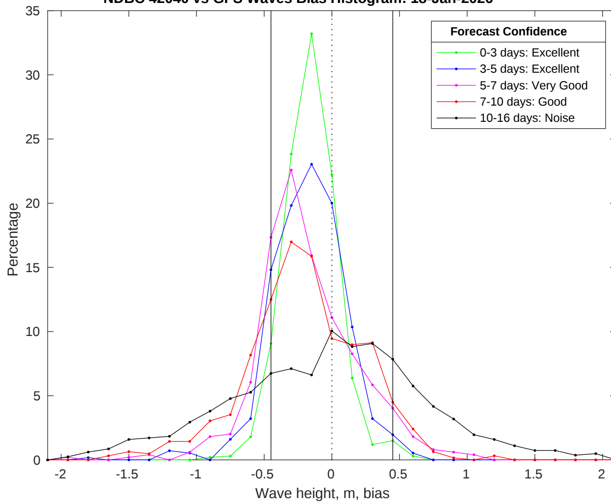
NDBC 42040 vs GFS Waves Bias Histogram: 18-Jan-2026
