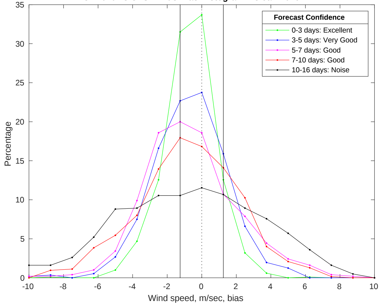
NDBC 42040 vs GFS Winds Bias Histogram: 18-Jan-2026
