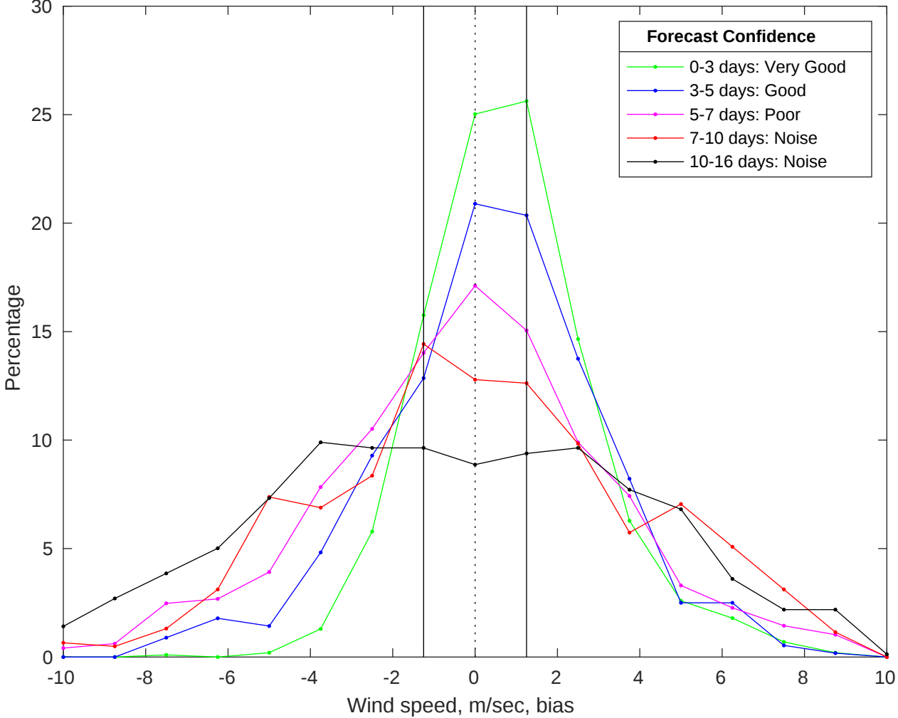
NDBC 44008 vs GFS Winds Bias Histogram: 18-Jan-2026
