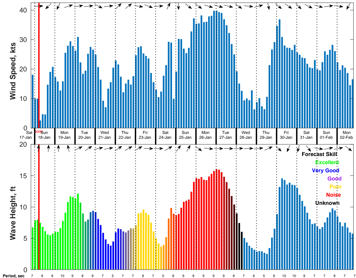
Wind & Wave Forecast for NDBC 44008 from 17-Jan-2026 20:00:00 to 02-Feb-2026 20:00:00
