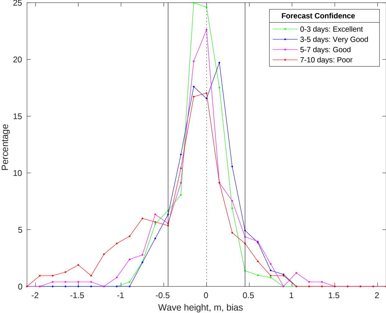
NDBC 46011 vs CMEMS Waves Bias Histogram: 18-Jan-2026
