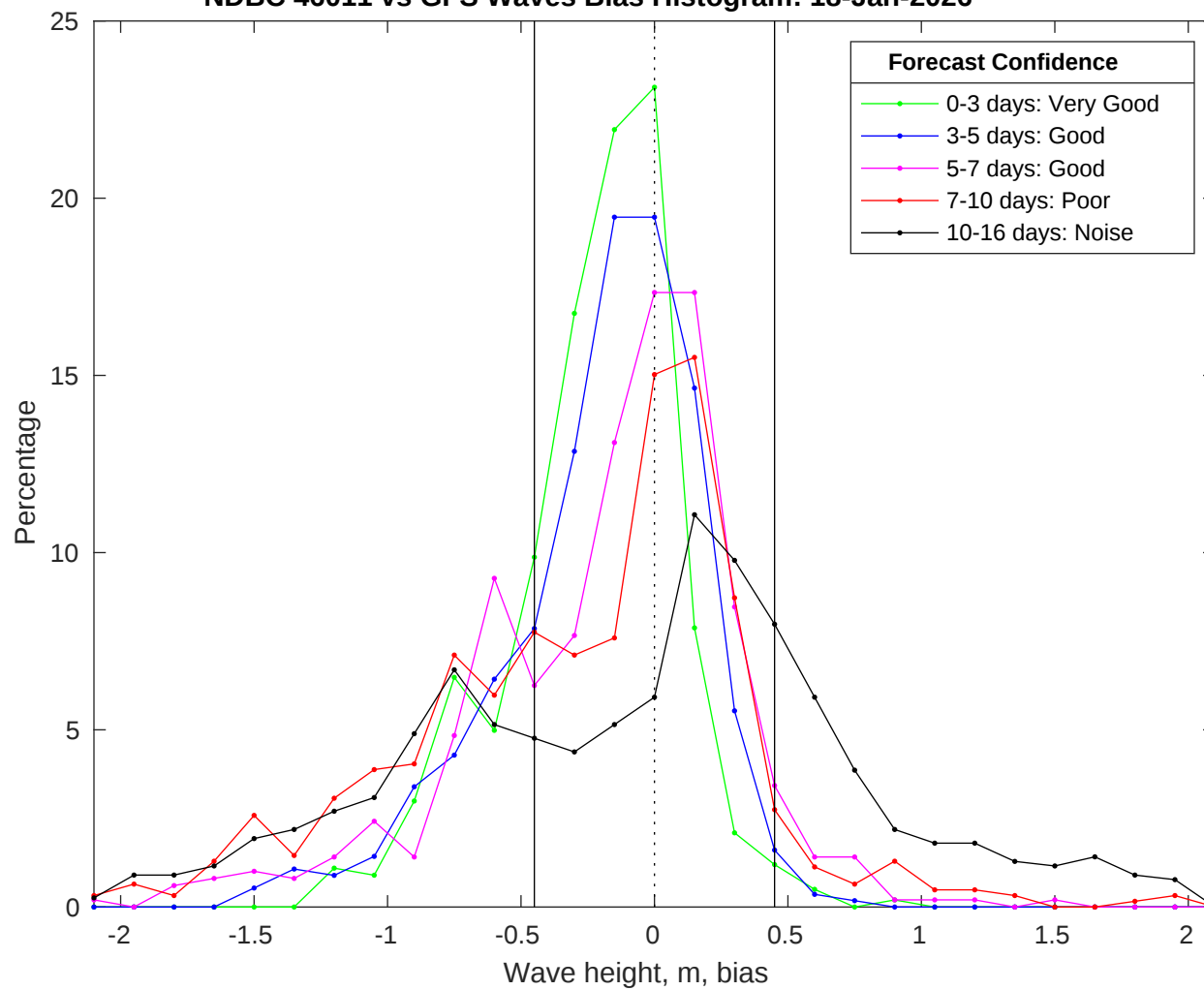
NDBC 46011 vs GFS Waves Bias Histogram: 18-Jan-2026
