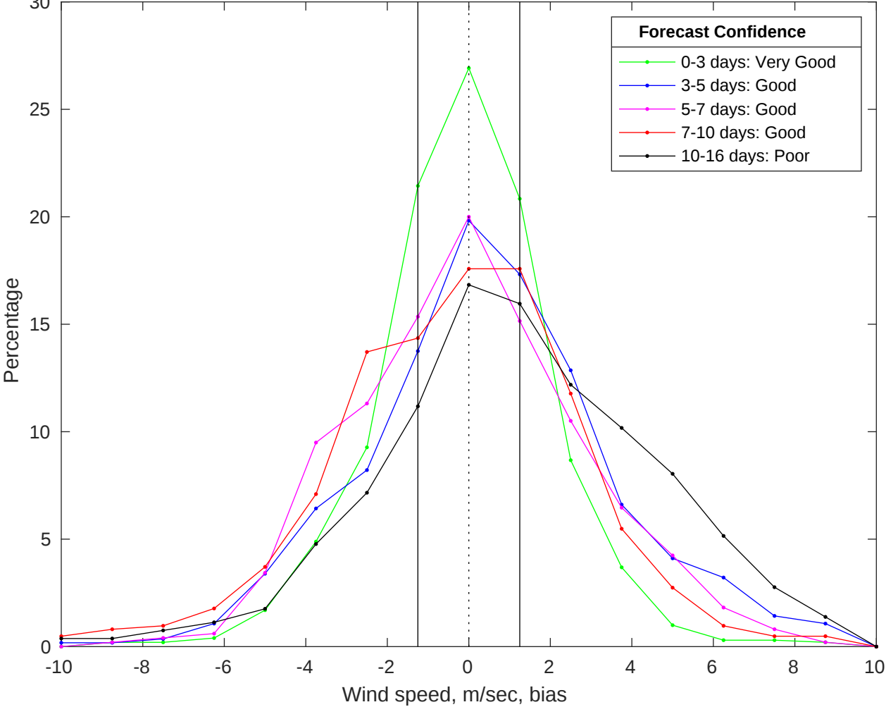
NDBC 46011 vs GFS Winds Bias Histogram: 18-Jan-2026
