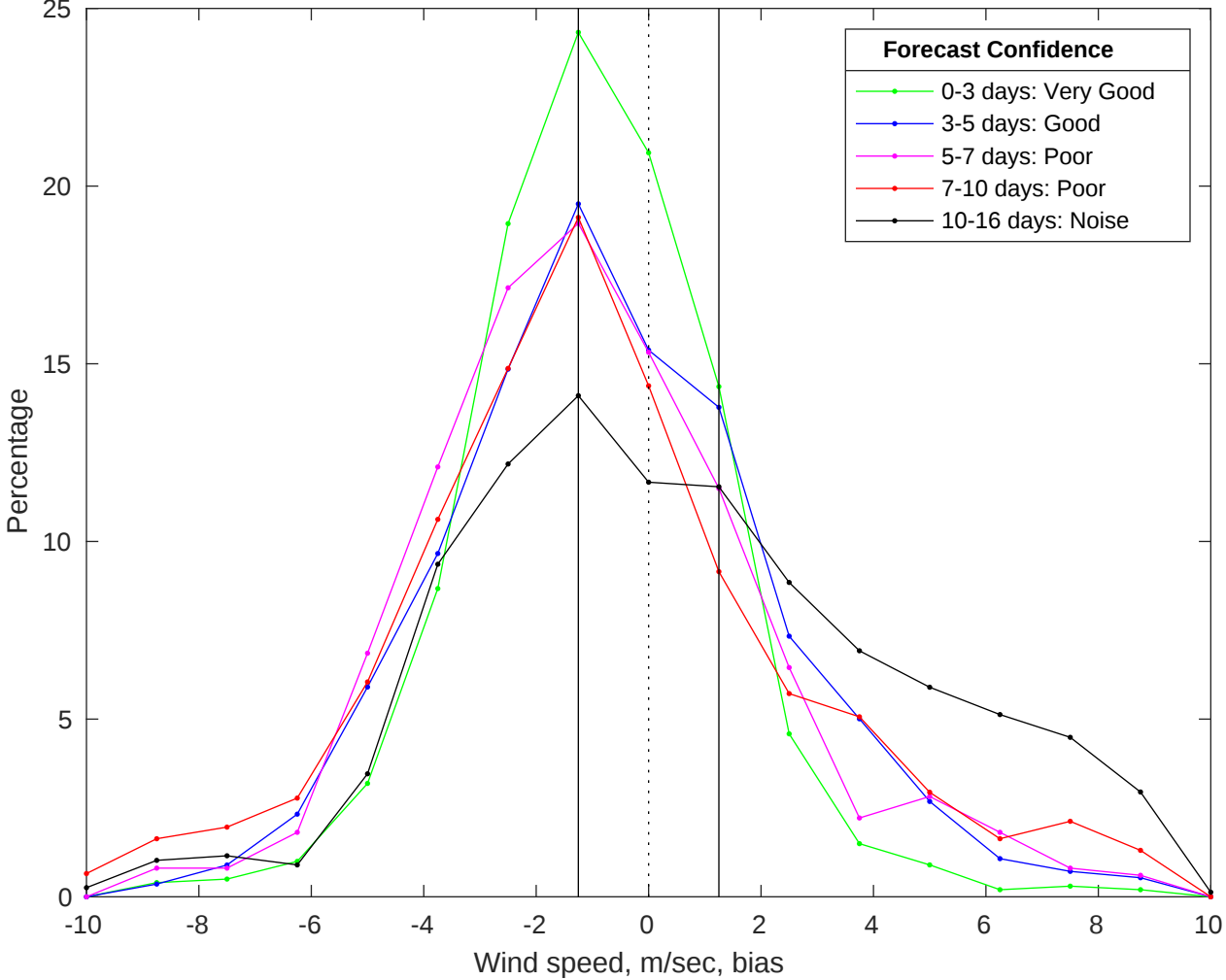
NDBC 46028 vs GFS Winds Bias Histogram: 18-Jan-2026
