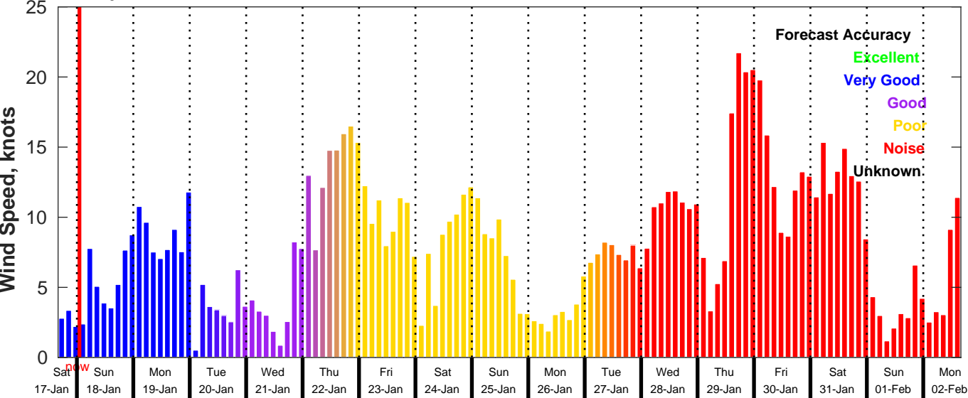
GFS Wind Speed Forecast for NDBC 46028 from 17-Jan-2026 16:00:00 to 02-Feb-2026 16:00:00
