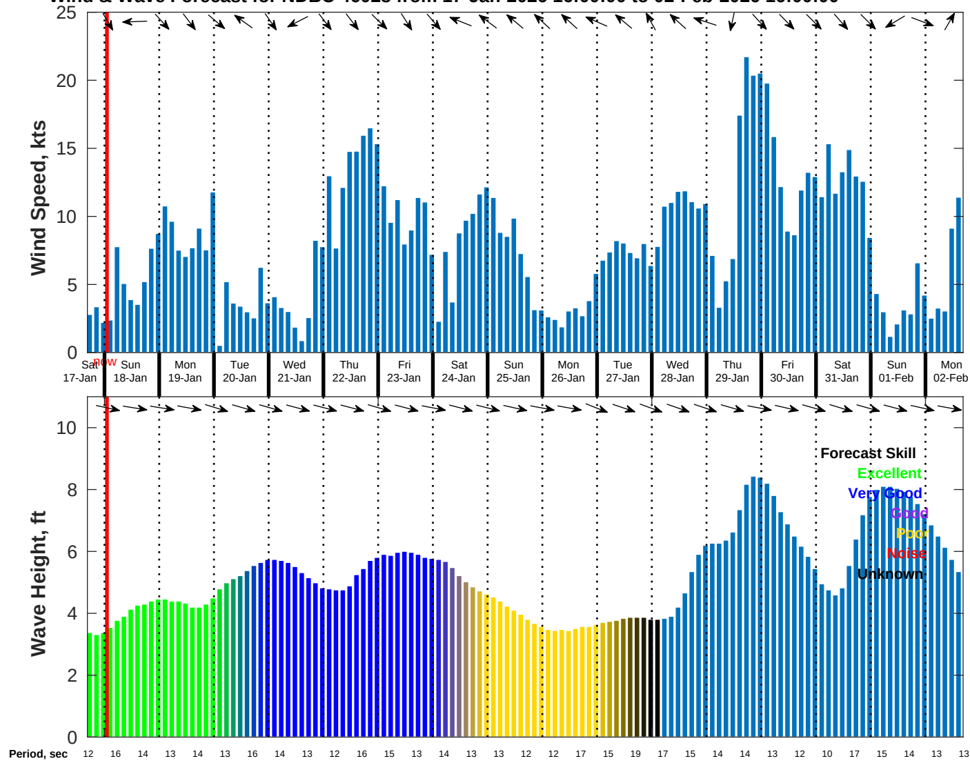
Wind & Wave Forecast for NDBC 46028 from 17-Jan-2026 16:00:00 to 02-Feb-2026 16:00:00
