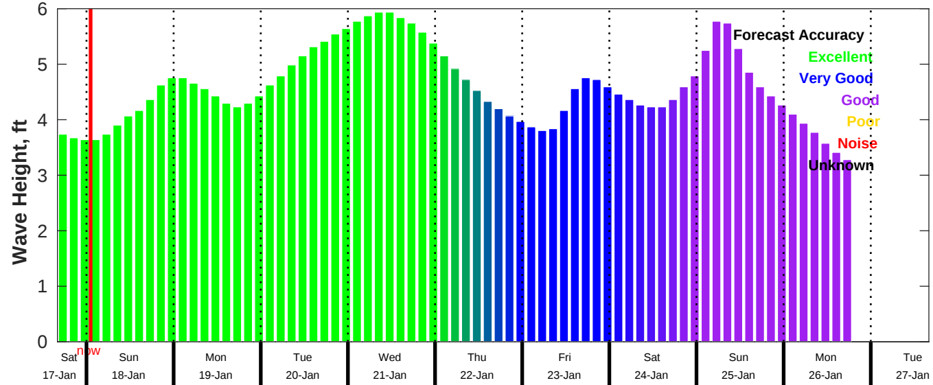
CMEMS Wave Forecast for NDBC 46054 from 17-Jan-2026 16:00:00 to 27-Jan-2026 16:00:00
