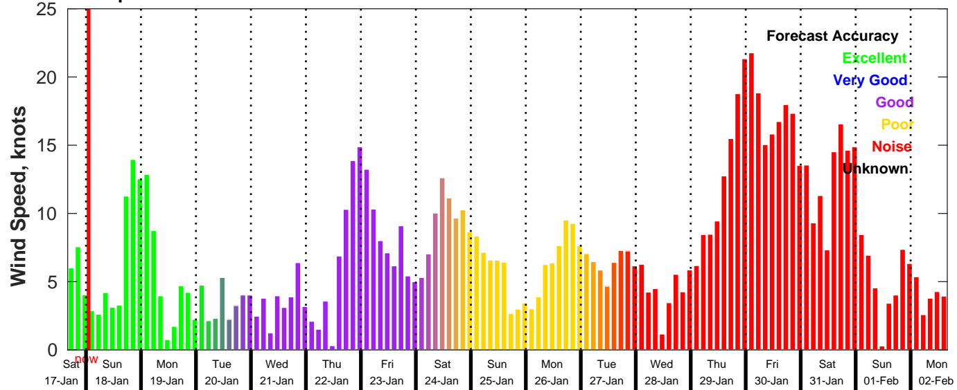
GFS Wind Speed Forecast for NDBC 46054 from 17-Jan-2026 16:00:00 to 02-Feb-2026 16:00:00
