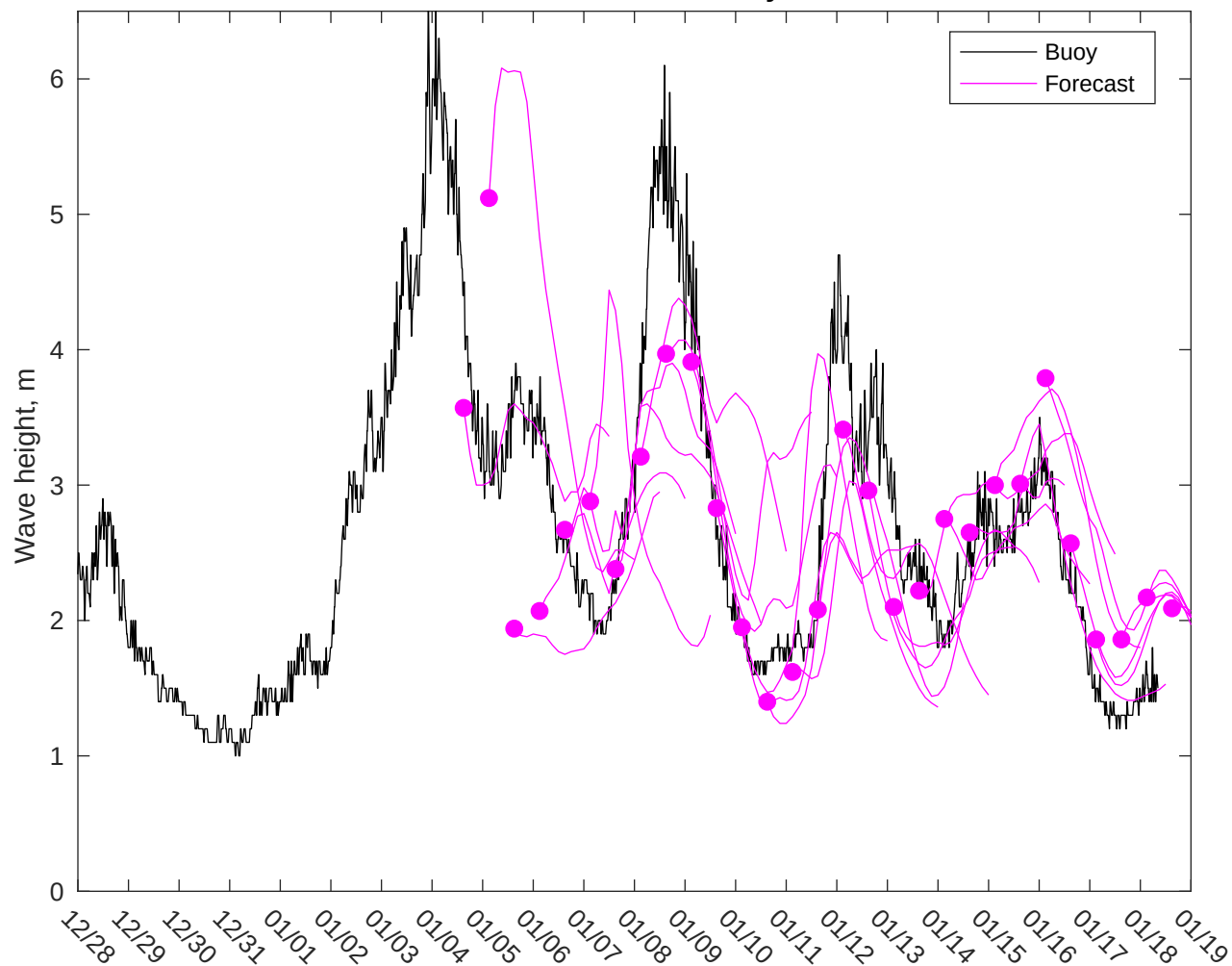
NDBC 46059 vs GFS Waves: 7 to 10 day forecast
