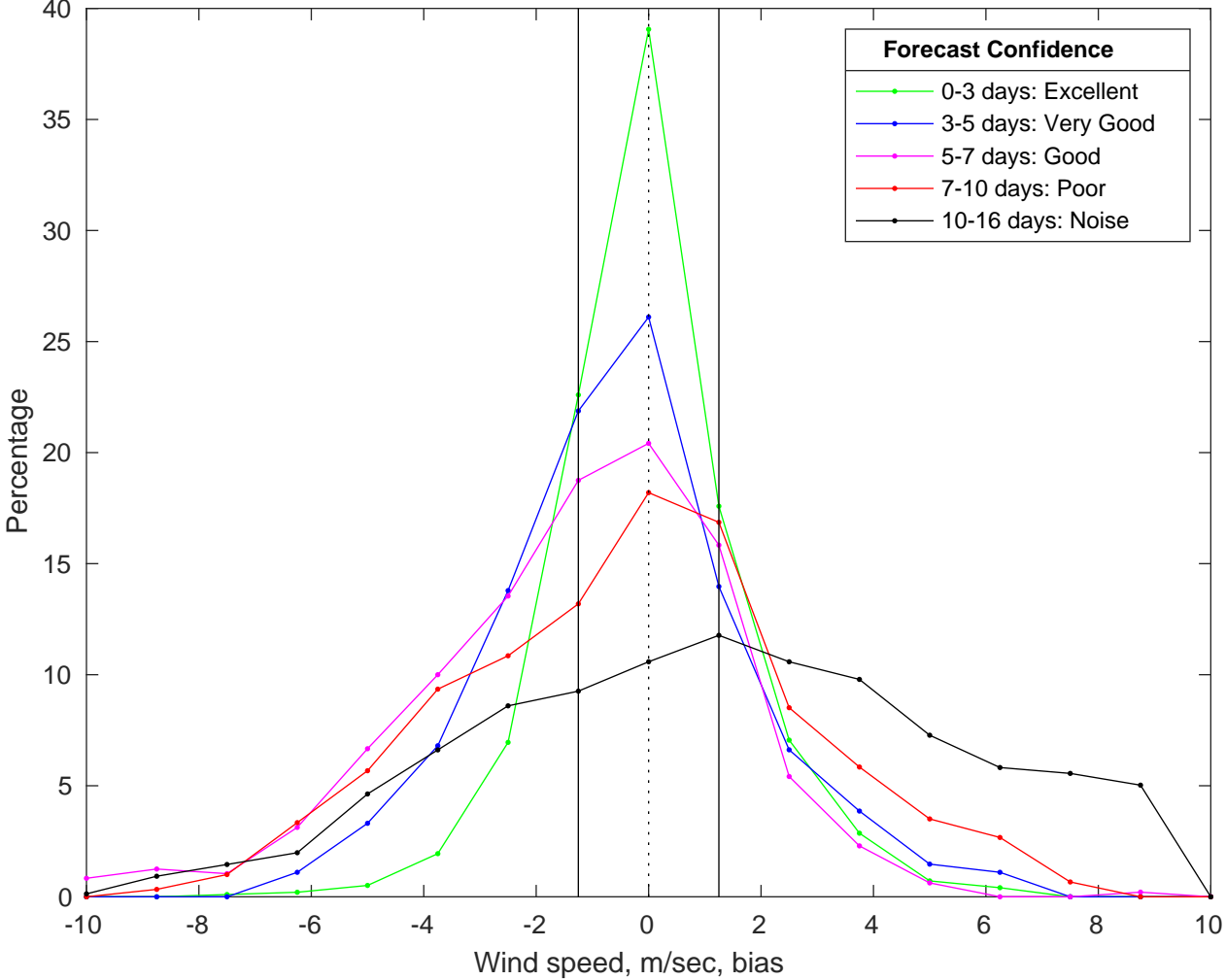
NDBC 46059 vs GFS Winds Bias Histogram: 18-Jan-2026
