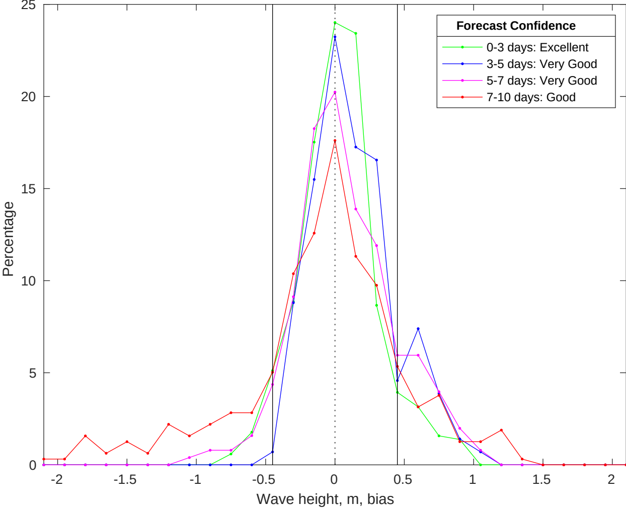
NDBC 46069 vs CMEMS Waves Bias Histogram: 18-Jan-2026
