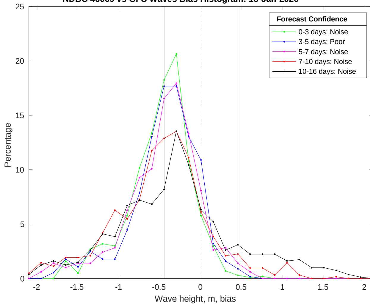
NDBC 46069 vs GFS Waves Bias Histogram: 18-Jan-2026
