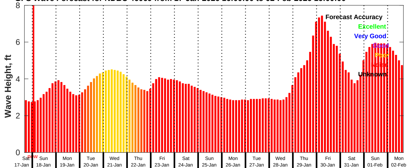
GFS Wave Forecast for NDBC 46069 from 17-Jan-2026 16:00:00 to 02-Feb-2026 16:00:00
