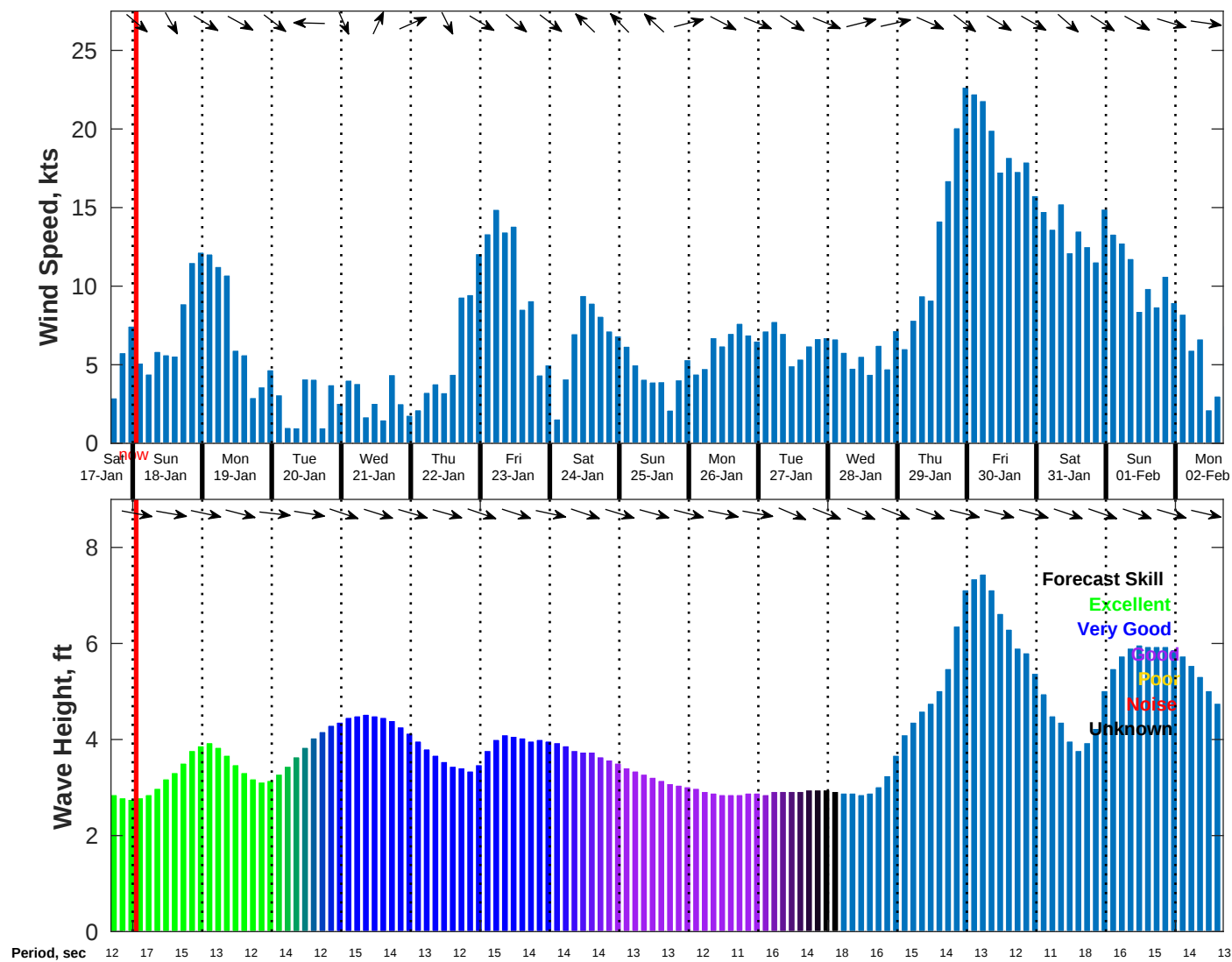
Wind & Wave Forecast for NDBC 46069 from 17-Jan-2026 16:00:00 to 02-Feb-2026 16:00:00
