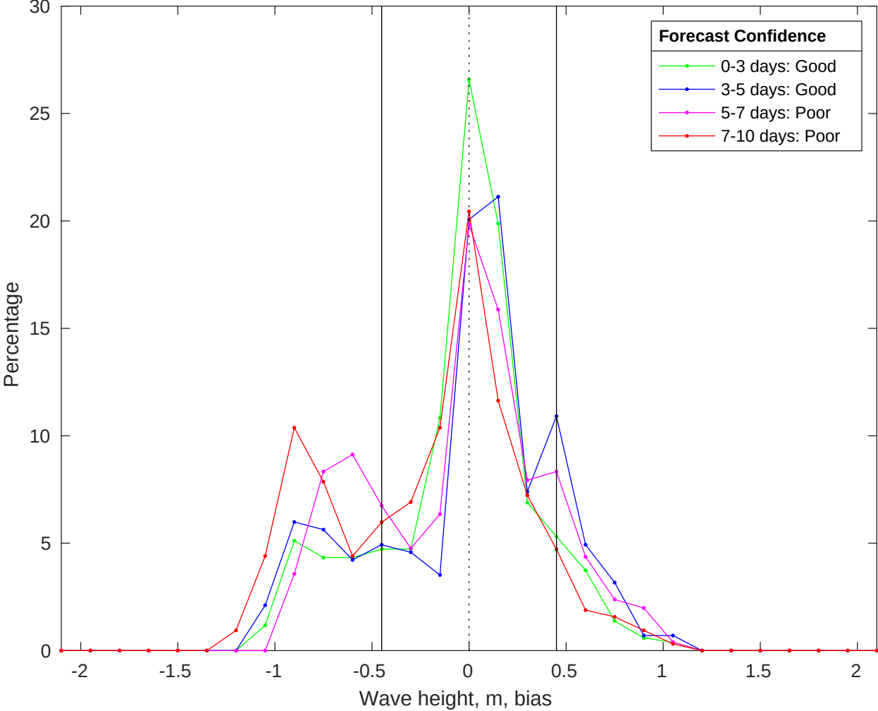
NDBC 46215 vs CMEMS Waves Bias Histogram: 18-Jan-2026
