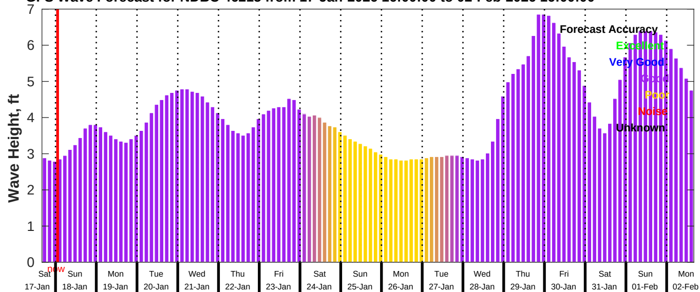
GFS Wave Forecast for NDBC 46215 from 17-Jan-2026 16:00:00 to 02-Feb-2026 16:00:00
