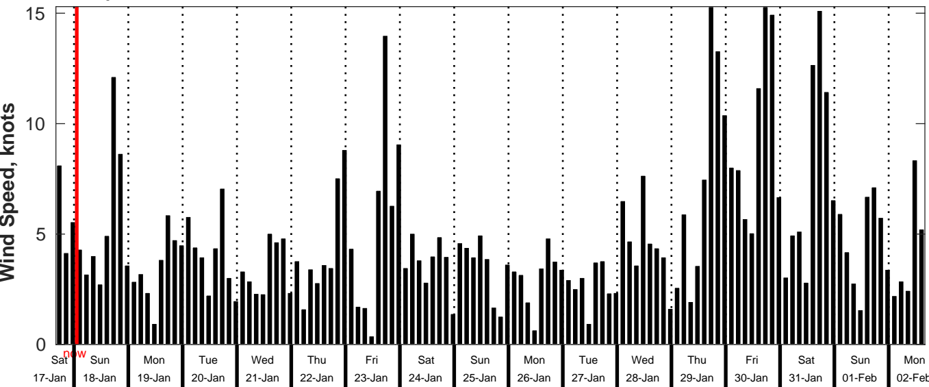
GFS Wind Speed Forecast for NDBC 46215 from 17-Jan-2026 16:00:00 to 02-Feb-2026 16:00:00
