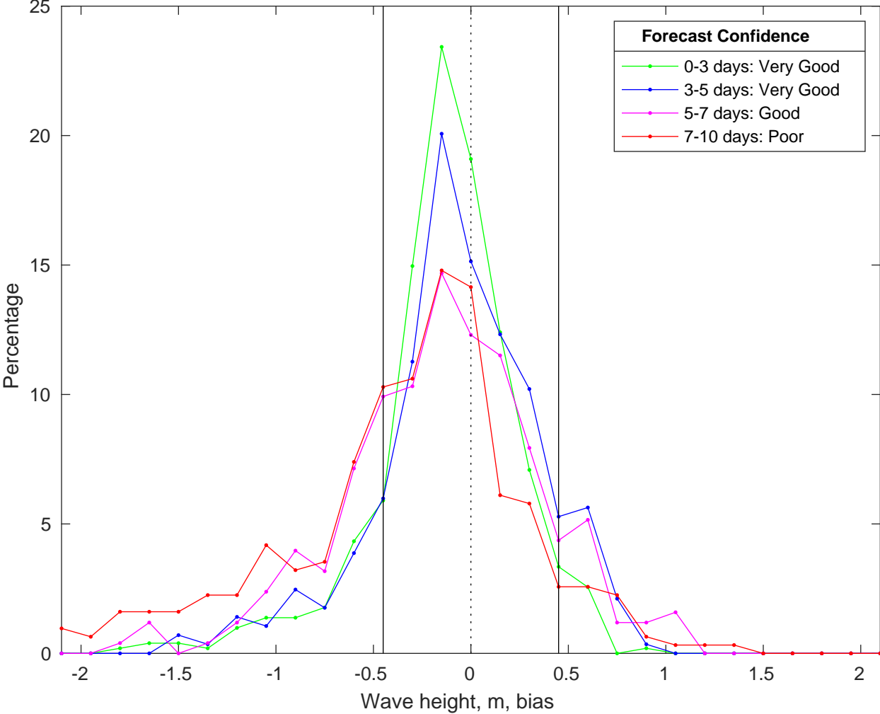
NDBC 46259 vs CMEMS Waves Bias Histogram: 18-Jan-2026
