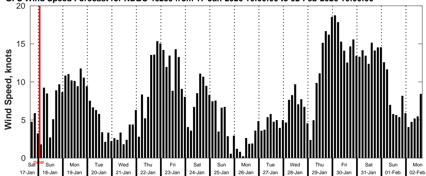
GFS Wind Speed Forecast for NDBC 46259 from 17-Jan-2026 16:00:00 to 02-Feb-2026 16:00:00
