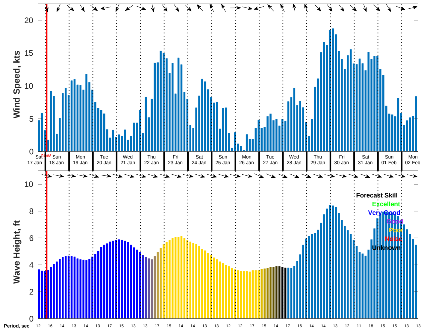
Wind & Wave Forecast for NDBC 46259 from 17-Jan-2026 16:00:00 to 02-Feb-2026 16:00:00
