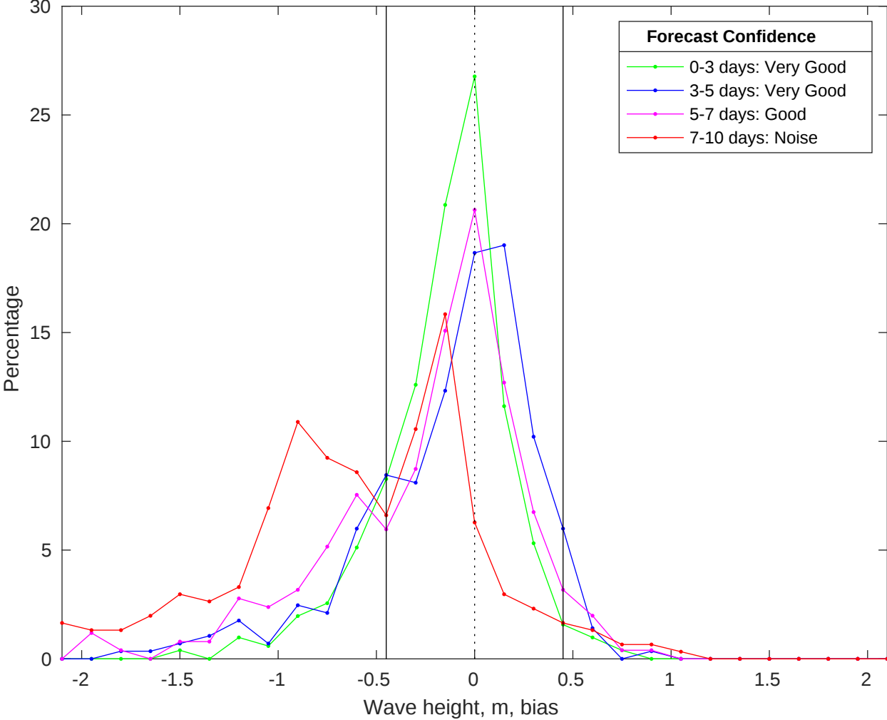
NDBC 51000 vs CMEMS Waves Bias Histogram: 18-Jan-2026
