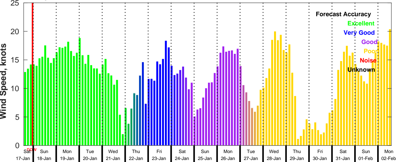
GFS Wind Speed Forecast for NDBC 51000 from 17-Jan-2026 14:00:00 to 02-Feb-2026 14:00:00
