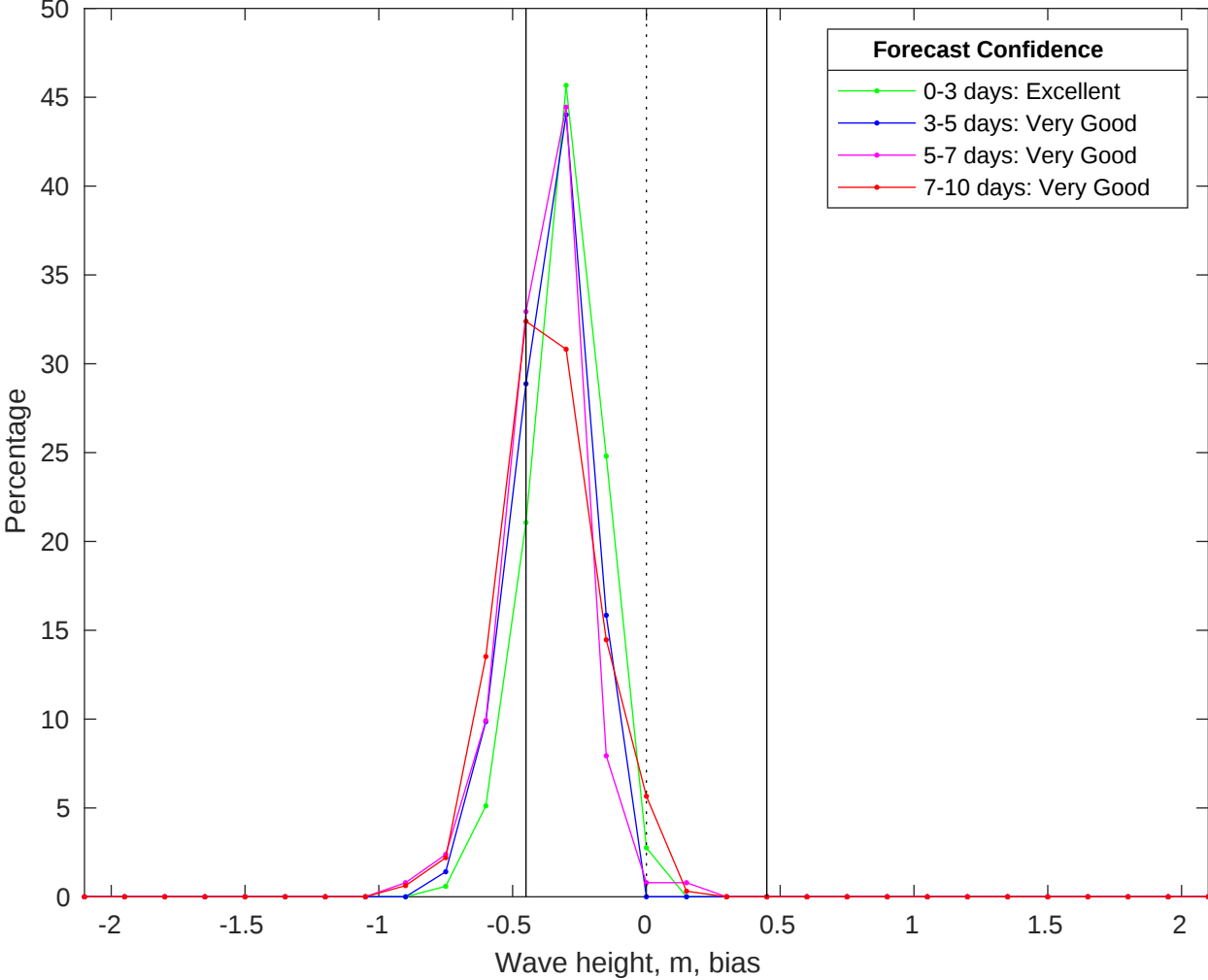
NDBC 51209 vs CMEMS Waves Bias Histogram: 18-Jan-2026
