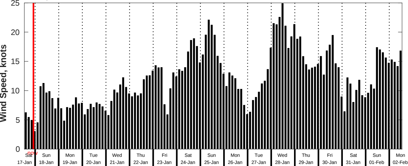
GFS Wind Speed Forecast for NDBC 51209 from 17-Jan-2026 13:00:00 to 02-Feb-2026 13:00:00
