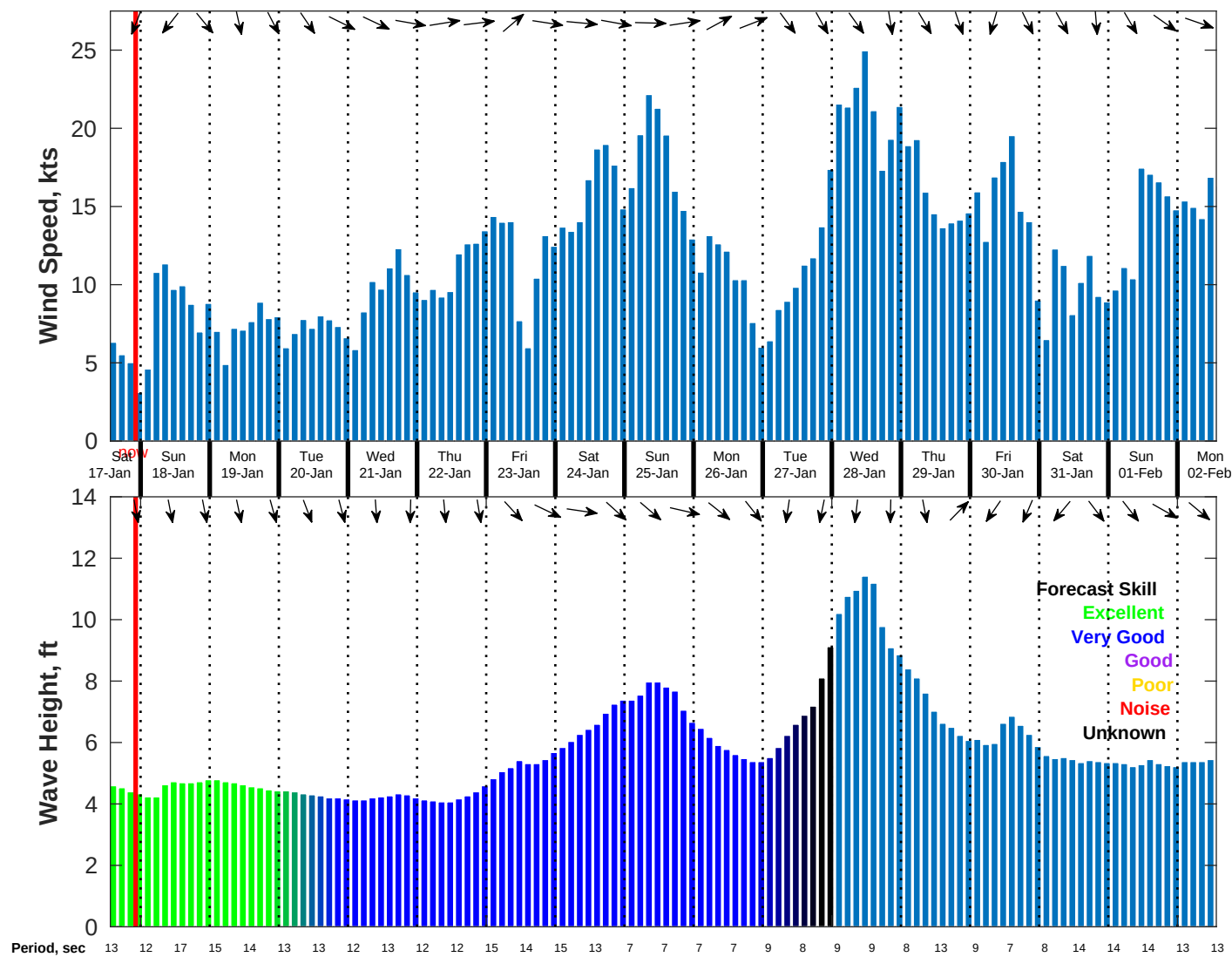
Wind & Wave Forecast for NDBC 51209 from 17-Jan-2026 13:00:00 to 02-Feb-2026 13:00:00
