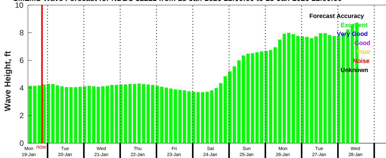
CMEMS Wave Forecast for NDBC 52211 from 18-Jan-2026 11:00:00 to 28-Jan-2026 11:00:00
