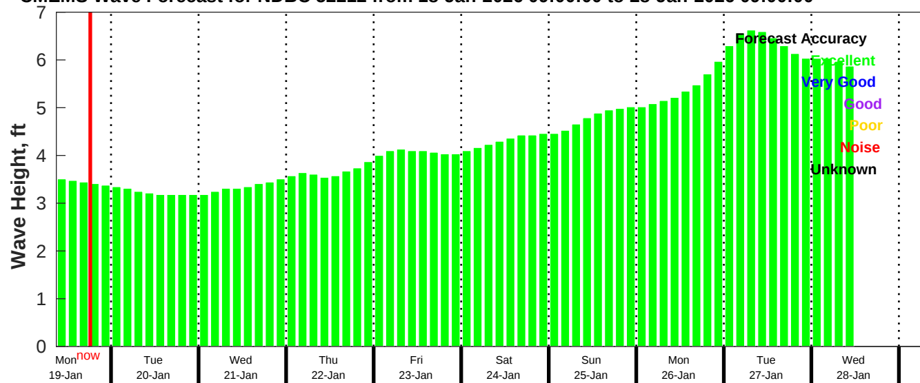
CMEMS Wave Forecast for NDBC 52212 from 18-Jan-2026 09:00:00 to 28-Jan-2026 09:00:00
