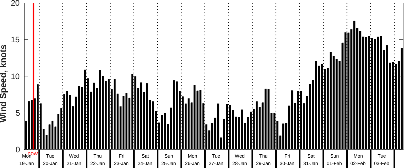
GFS Wind Speed Forecast for NDBC 52212 from 18-Jan-2026 09:00:00 to 03-Feb-2026 09:00:00
