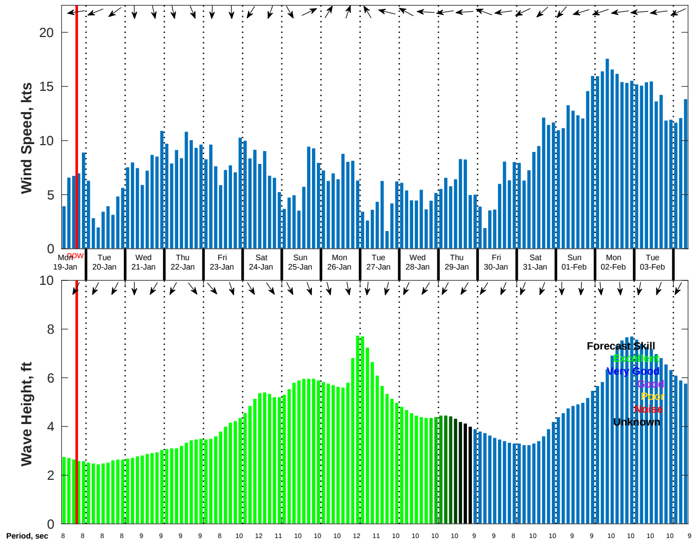
Wind & Wave Forecast for NDBC 52212 from 18-Jan-2026 09:00:00 to 03-Feb-2026 09:00:00
