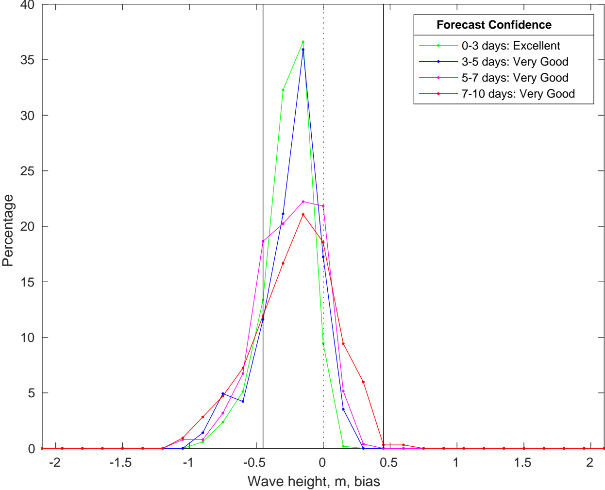
NDBC 52213 vs CMEMS Waves Bias Histogram: 18-Jan-2026
