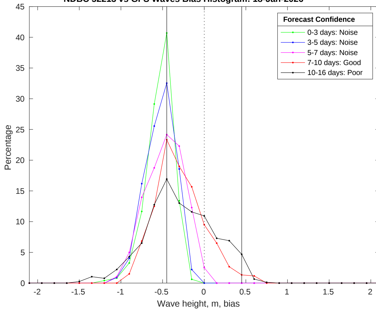
NDBC 52213 vs GFS Waves Bias Histogram: 18-Jan-2026
