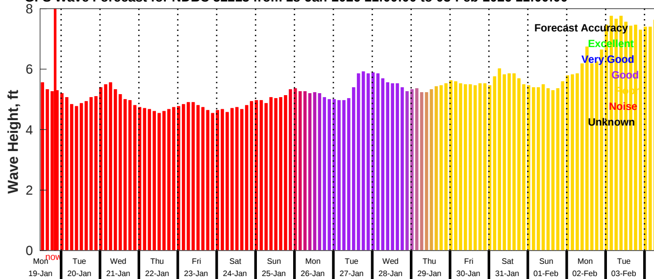
GFS Wave Forecast for NDBC 52213 from 18-Jan-2026 11:00:00 to 03-Feb-2026 11:00:00
