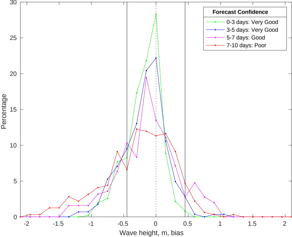
NDBC 41004 vs CMEMS Waves Bias Histogram: 19-Jan-2026
