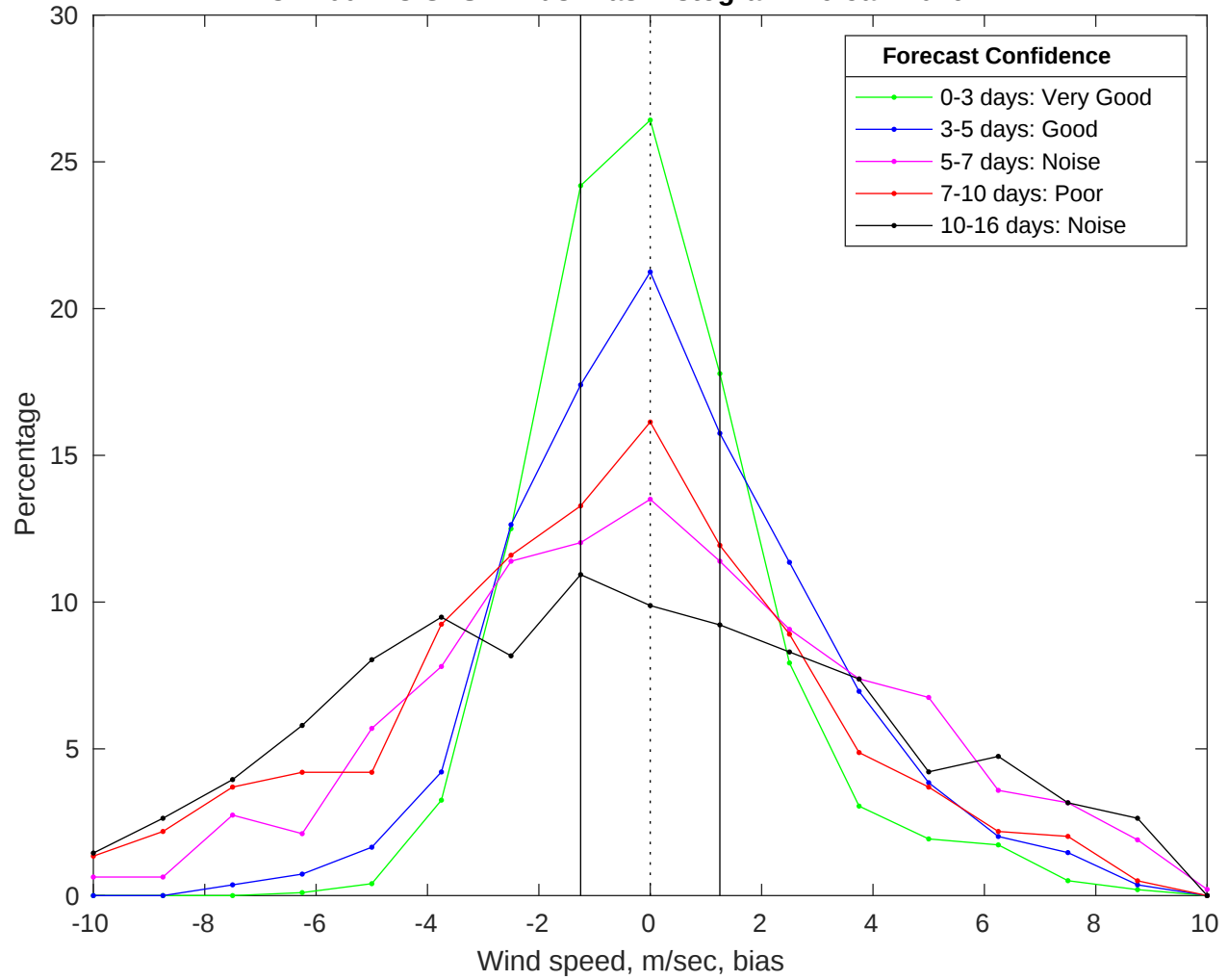
NDBC 41004 vs GFS Winds Bias Histogram: 19-Jan-2026
