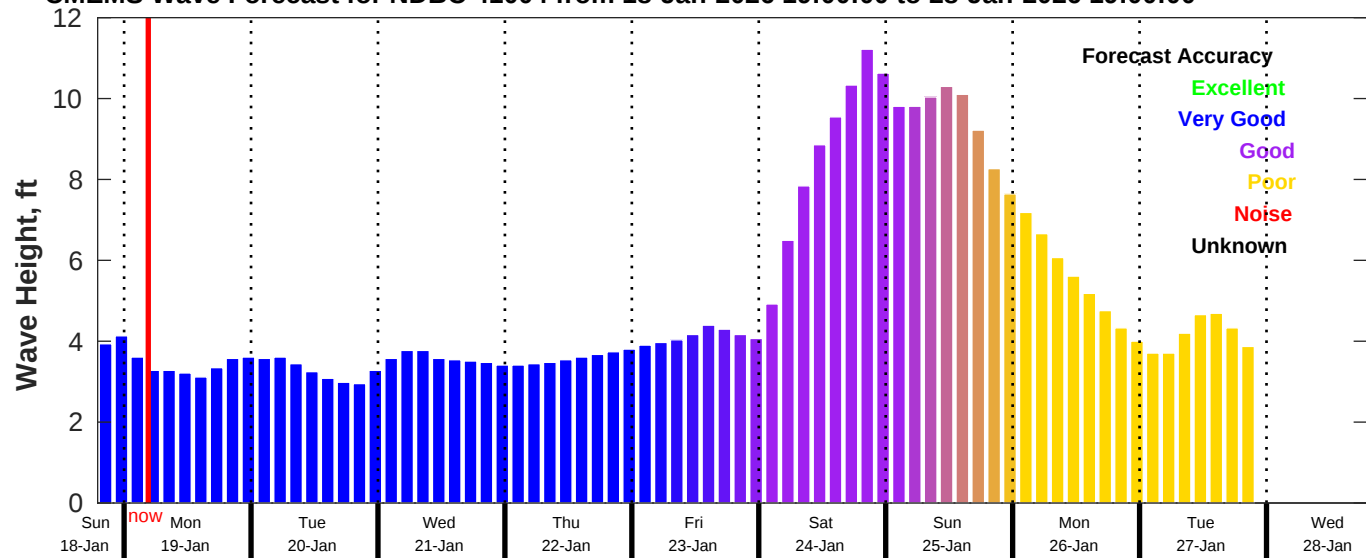
CMEMS Wave Forecast for NDBC 41004 from 18-Jan-2026 19:00:00 to 28-Jan-2026 19:00:00
