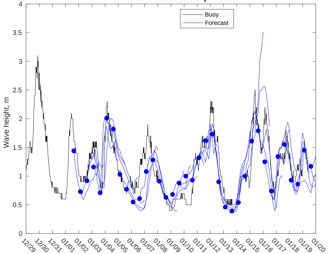
NDBC 41013 vs GFS Waves: 3 to 5 day forecast
