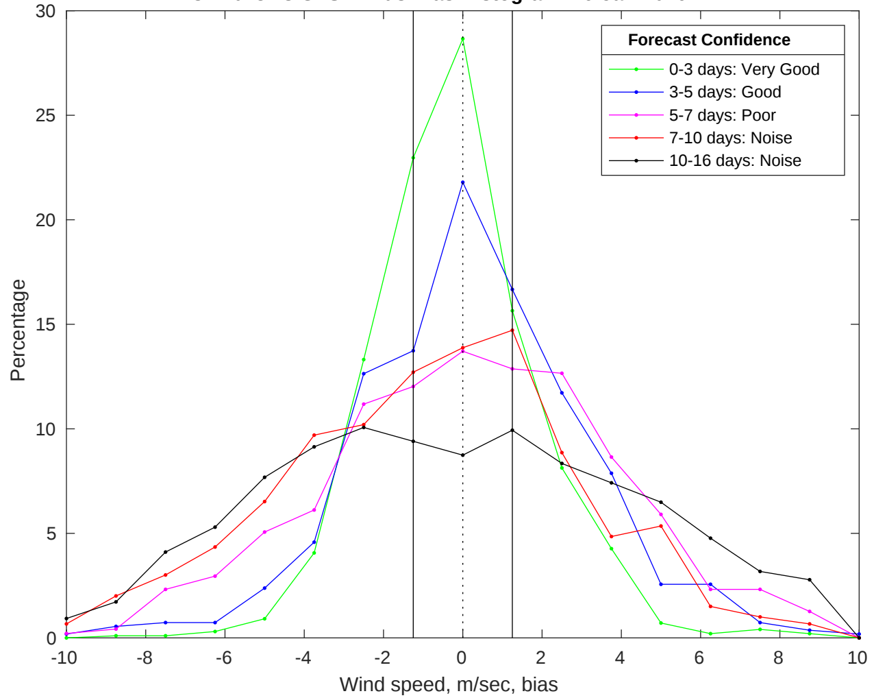
NDBC 41013 vs GFS Winds Bias Histogram: 19-Jan-2026
