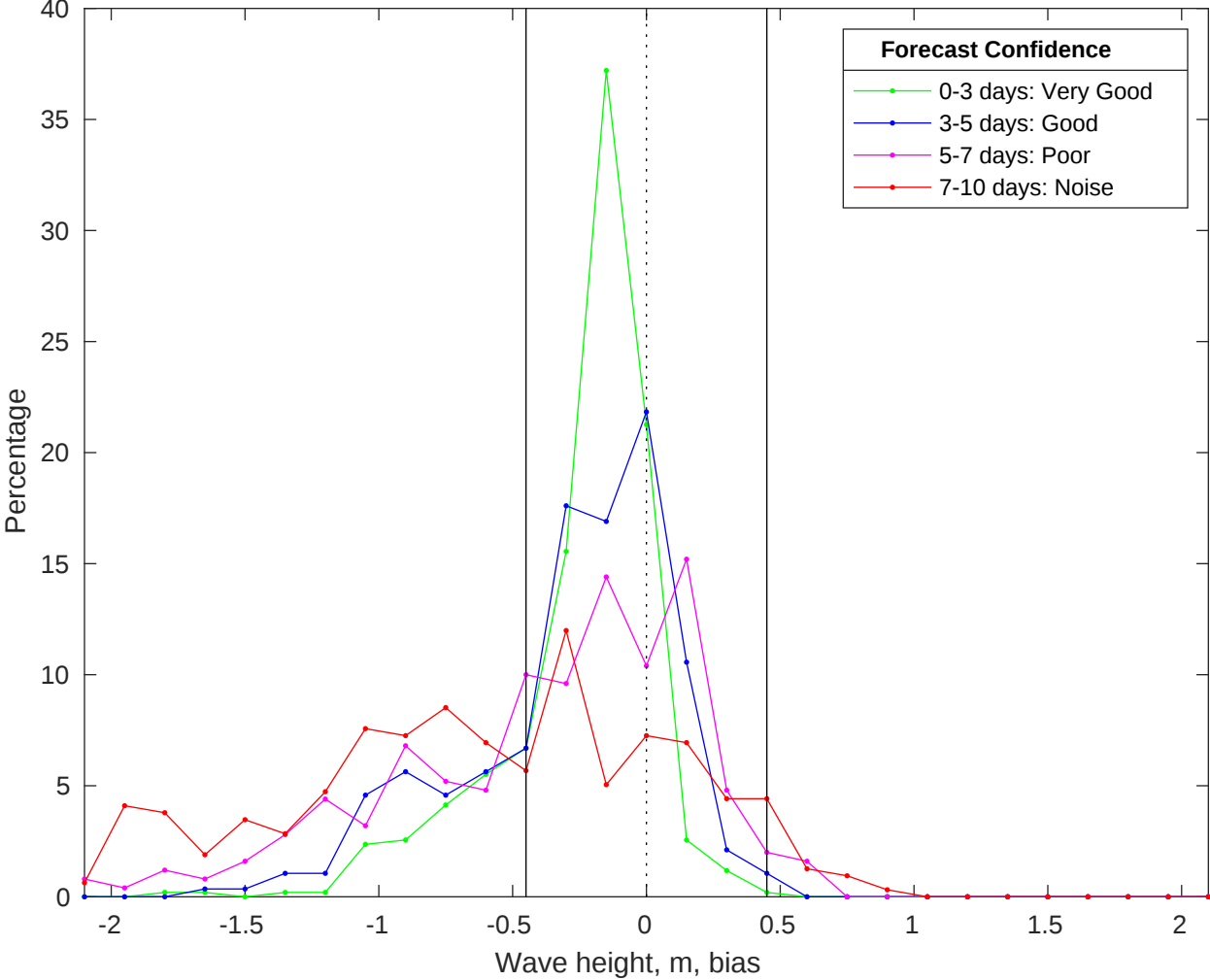
NDBC 42019 vs CMEMS Waves Bias Histogram: 19-Jan-2026
