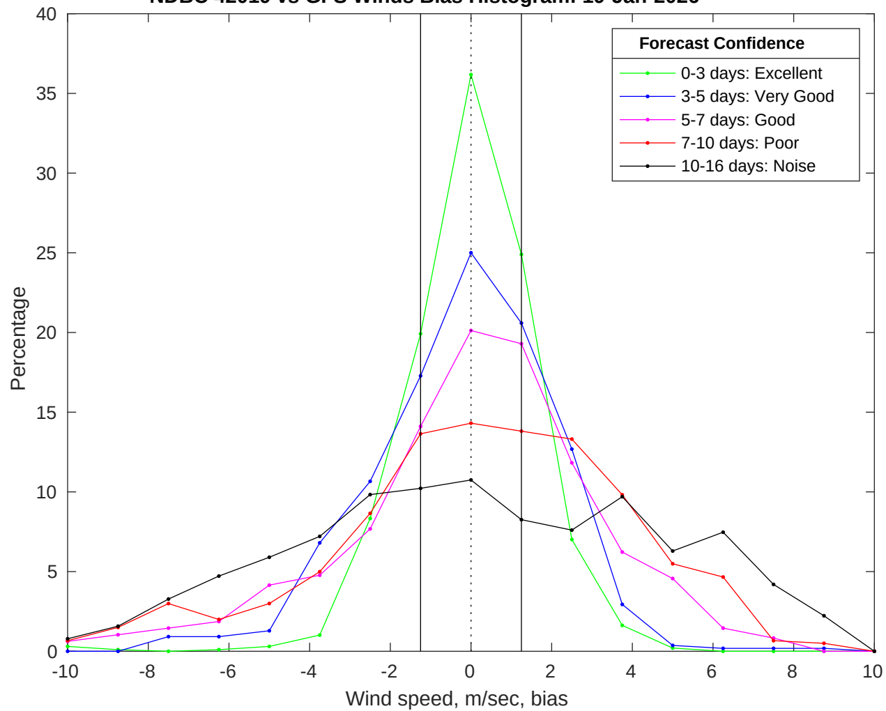
NDBC 42019 vs GFS Winds Bias Histogram: 19-Jan-2026
